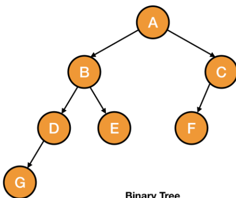
Binary Tree
