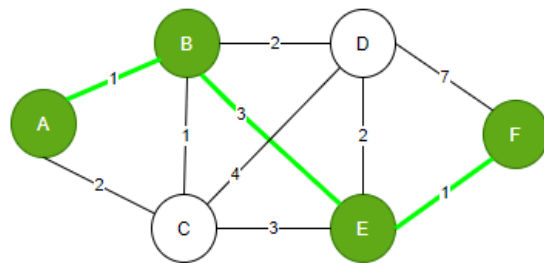
Weighted Graph
